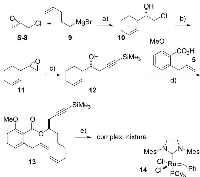
Scheme 1. Synthesis of the benzoate 13 and its attempts to cyclize it to the corresponding macrolactone; a) bromopentene (1 equiv.), THF, Mg (1.38 equiv.), 50 °C, add to CuCN (0.04 equiv.), S-8 (0.77 equiv.), THF, –50 °C, 2 h, 100 %; b) NaOH (2 equiv.), ethylene glycol, 0 to 23 °C, 1 h, 73 %; c) Me 3 SiCCH (1 equiv.), n BuLi (0.93 equiv.), THF, –78 °C, 30 min, add BF 3 ·Et 2 O (1 equiv.), 30 min, add 11 (0.64 equiv.), –78 °C, 3 h, 36 %; d) 12 (1 equiv.), Ph 3 P (2.5 equiv.), acid 5 (5 equiv.), DIAD (2.5 equiv.), toluene, 23 °C, 3 h, 65 %. DIAD = diisopropylazodicarboxylate.
