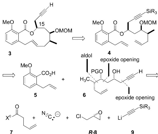
Figure 2. Retrosynthetic analysis of the propynyl-substituted macrolactone 3 leading to epichlorohydrin as starting material; R = alkyl, PG = non-silyl protecting group, X c = chiral auxiliary.
