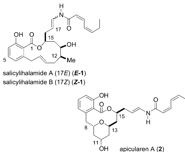
Figure 1. Structures of two important benzolactone enamides.
