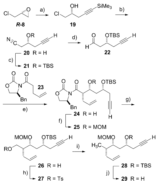
Scheme 3. Synthesis of the enynol 29 from epichlorohydrin R-8 ; a) \text{Me}_3\text{SiCCH} (1 equiv.), n\text{BuLi} (0.93 equiv.), -78^\circ\text{C} , 30 min, then add \text{BF}_3 \cdot \text{Et}_2\text{O} (1 equiv.), -78^\circ\text{C} , 30 min, then add R-8 (0.64 equiv.), -78^\circ\text{C} , 3 h, (98 %); [24b] b) \text{NaCN} (2.5 equiv.), \text{EtOH} , 23^\circ\text{C} , 3 d, 96 %; c) t\text{BuMe}_2\text{SiCl} (1.5 equiv.), imidazole (2.5 equiv.), DMAP (0.05 equiv.), \text{DMF} , 23^\circ\text{C} , 3 d, 100 %; d) DIBAL (1.2 equiv.), \text{CH}_2\text{Cl}_2 , -78^\circ\text{C} , 4 h, 96 %; e) compound 23 (1 equiv.), \text{TiCl}_4 (1.05 equiv.), (–)-sparteine (2.5 equiv.), \text{CH}_2\text{Cl}_2 , 0^\circ\text{C} , 20 min, add aldehyde 22 (1.27 equiv.), 0^\circ\text{C} , 1 h, 89 %; f) i\text{Pr}_2\text{NEt} (10 equiv.), \text{MeOCH}_2\text{Cl} (5 equiv.), \text{Bu}_4\text{NI} (0.2 equiv.), 0 to 23^\circ\text{C} , 24 h, 80 %; g) \text{LiBH}_4 (1.3 equiv.), \text{EtOH} (1.3 equiv.), \text{Et}_2\text{O} , 0 to 23^\circ\text{C} , 12 h, 68 %; h) p\text{TsCl} (3 equiv.), pyridine, 0^\circ\text{C} , 5 h, 100 %; i) \text{Et}_3\text{BHLi} (5 equiv.), \text{THF} , 0 to 23^\circ\text{C} , 93 %; j) TBAF (2 equiv.), \text{THF} , 0 to 23^\circ\text{C} , 84 %.
