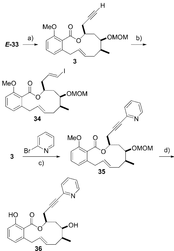
Scheme 5. Synthesis of the vinyl iodide 34 and the salicylihalamide analog 36 from the macrolactone E-33 ; a) TBAF (4.8 equiv.), THF, 23 °C, 5 h, 94 %; b) Bu 3 SnH (1.2 equiv.), AIBN (0.13 equiv.), toluene, reflux, 18 h, change solvent to Et 2 O, add I 2 (1.2 equiv.), 0 °C, 1 h, 83 % ( E/Z = 3.8:1); c) bromopyridine (0.92 equiv.), [PdCl 2 (PPh 3 ) 2 ] (0.022 equiv.), CuI (0.045 equiv.), Et 3 N, 23 °C, 18 h, 90 %; d) 9-I-9-BBN (4 equiv.), CH 2 Cl 2 , 23 °C, 70 s, 88 %. 9-I-9-BBN = 9-Iodo-9-borabicyclo[3.3.1]nonane.
