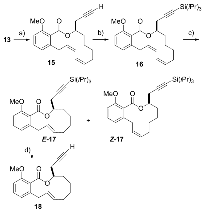
Scheme 2. Synthesis of the benzoate 16 with a TIPS-protected alkyne and its ring closing metathesis to the macrolactones 17 ; a) K 2 CO 3 (2 equiv.), MeOH, 23 °C, 4 h, 85 %; b) n BuLi (1.12 equiv.), THF, –78 to –20 °C, 30 min, then add ( i Pr) 3 SiCl (1.2 equiv.), THF, –78 to 23 °C, 15 h, 78 %; c) catalyst 14 (0.05 equiv.), toluene, 75 °C, 2 h, 99 % ( E/Z = 4.21:1); d) TBAF (5 equiv.), THF, 0 to 23 °C, 5 h, (100 %).
